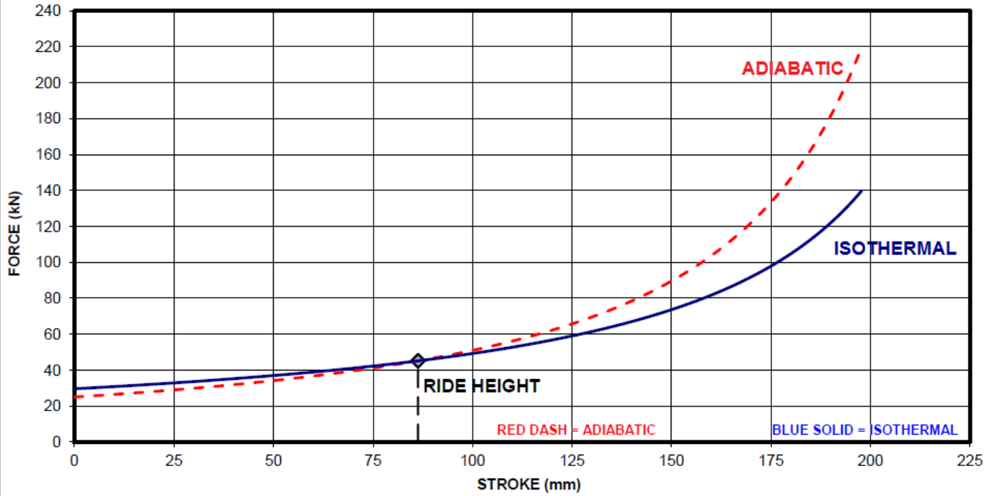
TYPICAL ISOTHERMAL AND ADIABATIC SPRING CURVE
