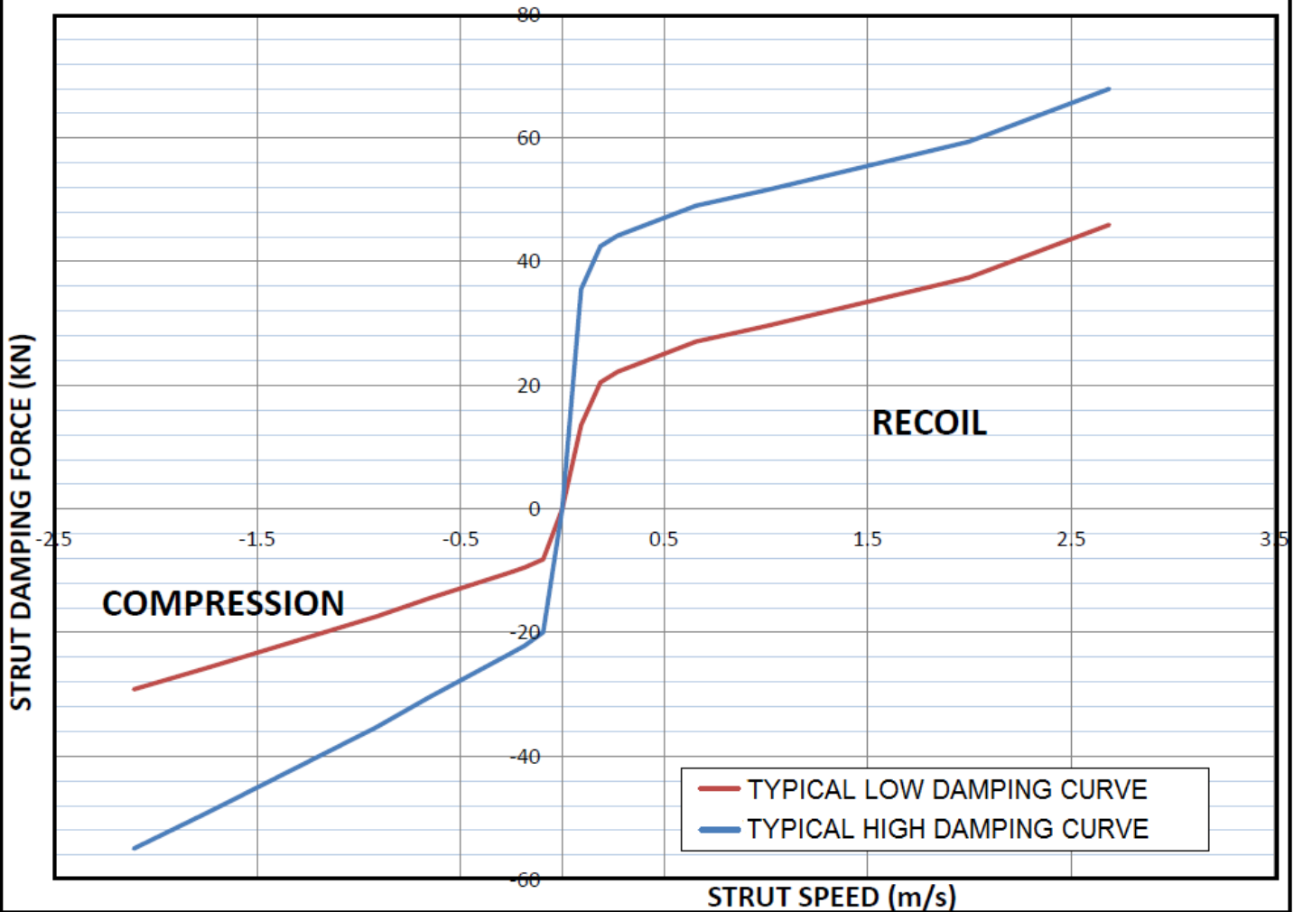
TYPICAL DAMPING FOR W-STRUT
